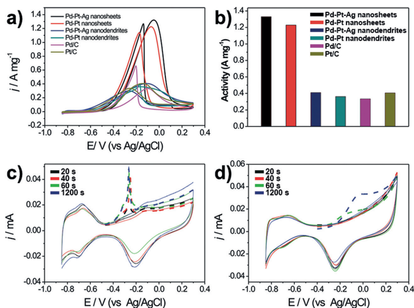
Figure 4. a) CVs obtained with various catalysts in 0.1 M KOH and 0.5 M ethanol at a scan rate of 50 mV s -1 . b) Catalytic activities of the different materials in the EOR. c, d) CO stripping voltammograms for the Pd-Pt (c) and Pd-Pt-Ag nanosheets (d) in 0.1 M KOH at a scan rate of 50 mV s -1 . The first and second scans are depicted as dashed and solid lines, respectively. Before the CO stripping tests, the working electrodes were held at -0.1 V vs. Ag/AgCl during CO purging for the indicated periods of time.
